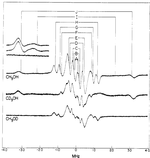
Figure 2. Proton ENDOR spectra of the \text{VO}^{2+} ion in methanol. \mathbf{H}_0 was set at the -7/2 \parallel EPR resonance feature ( \sim 2800 G). The samples were prepared in \text{CH}_3\text{OH} , \text{CD}_3\text{OH} , and \text{CH}_3\text{OD} solvents. The ENDOR absorption features are identified in the stick diagram and are equally spaced about the free-proton frequency of 11.88 MHz. The line pairs are identified in Tables I and II. For ENDOR features near the free-proton frequency, a modulation depth no greater than 30 kHz of the rf field was required to achieve maximum spectral resolution. The spectra at apparent higher gain in the upper left-hand part were recorded with a modulation depth of approximately 90 kHz.
