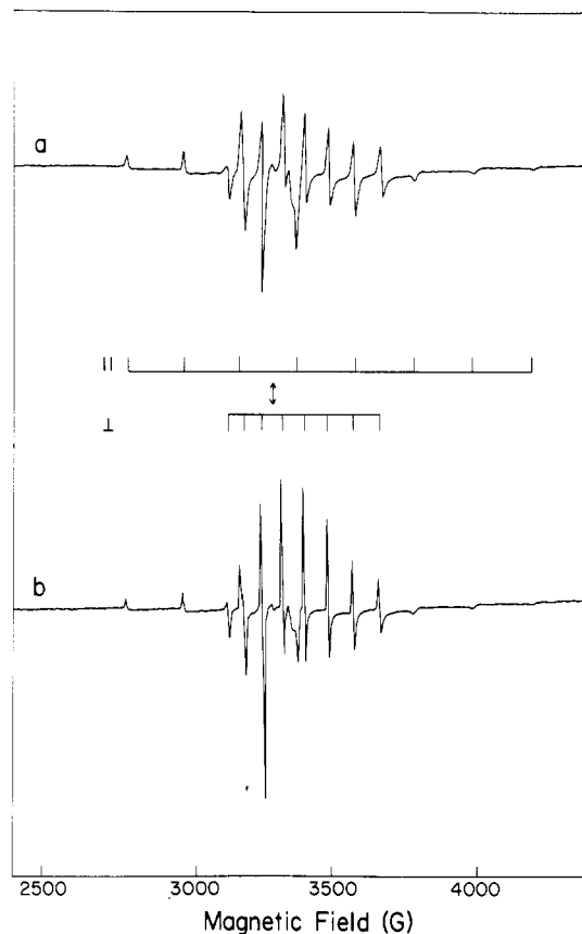
Figure 1. First-derivative EPR absorption spectra of VO 2+ in (a) 50:50 (v/v) CH 3 OH–H 2 O and (b) 50:50 CD 3 OD–D 2 O solvent mixtures. The spectra were recorded as described under Experimental Methods with the samples at 15 K and with 83.4 μW of incident microwave power modulated at 12.05 kHz. The modulation amplitude was 1.25 G pp . The parallel (||) and perpendicular (⊥) EPR absorption components (–7/2, –5/2, ..., 5/2, 7/2) are identified in sequence in the low- to high-field direction. The double-headed arrow indicates the magnetic field position corresponding to forbidden Δ M = ±1 transitions. 20
