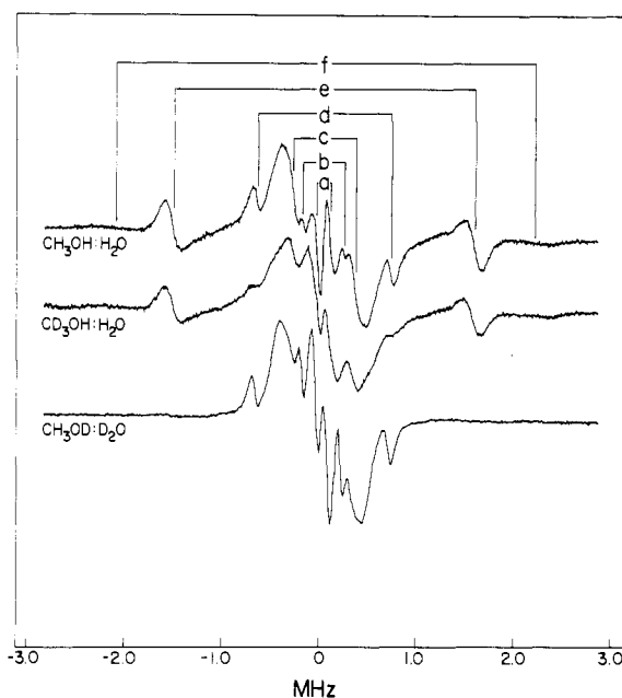
Figure 7. Proton ENDOR spectra of the VO 2+ ion in 50% aqueous methanol. H_0 was set to the -3/2 \perp EPR absorption ( \sim 3270 G). Six line pairs are seen equally spaced about the free-proton frequency (13.88 MHz) and are identified in Table V. Other conditions are as in Figure 3.
