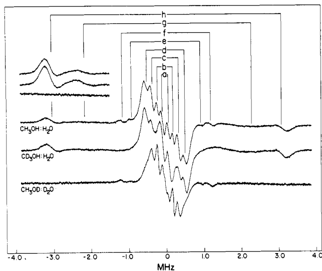
Figure 6. Proton ENDOR spectra of the VO 2+ ion in 50% water-methanol. H_0 was set to the -7/2 \parallel EPR absorption feature ( \sim 2800 G). The VO 2+ complexes were prepared as indicated in the following 50:50 (v/v) solvent mixtures: CH 3 OH-H 2 O, CD 3 OH-H 2 O, and CH 3 OD-D 2 O. The ENDOR lines of each pair are identified in the stick diagram and are seen to be equally spaced about the free-proton frequency of 11.84 MHz. The line pairs are identified in Table V. Other conditions are as in Figure 2.
