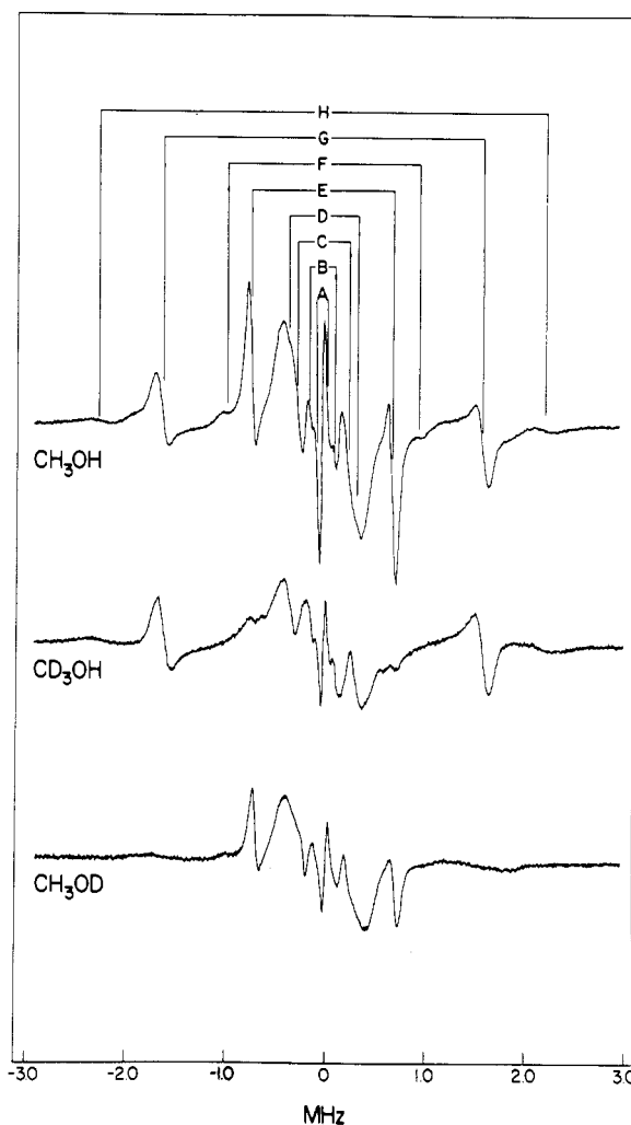
Figure 3. Proton ENDOR spectra of the \text{VO}^{2+} ion in methanol. \mathbf{H}_0 was set to the -3/2 \perp EPR resonance feature ( \sim 3270 G). Eight line pairs are seen equally spaced about the free-proton frequency 13.88 MHz and are identified in Tables I and II. A modulation depth of 10 kHz of the rf field was required to achieve maximum spectral resolution. Other conditions are as in Figure 2.
