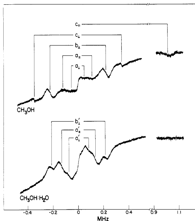
Figure 8. 13 C ENDOR spectra of the VO 2+ ion in methanol and aqueous methanol mixtures. H 0 was set to the -3/2 \perp EPR absorption. The lower frequency component belonging to line pair c || was not detectable as expected in the 1.5-2.5-MHz region because of a severely sloping base line. For both types of solvent systems, methanol enriched to 50% mole fraction 13 C was employed to ensure that the relative enrichment of metal-bound methanol molecules remained constant. The modulation depth of the rf field was 30 kHz. Other conditions are as in Figure 3.
