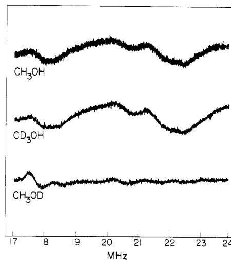
Figure 4. Proton ENDOR spectra of the \text{VO}^{2+} in methanol with the \mathbf{H}_0 setting at the -3/2 \perp EPR resonance feature. These ENDOR lines observed at higher frequency are due to a much larger isotropic hfc component than for those in Figure 3. A modulation depth of 70 kHz of the rf field was employed. Other conditions are as in Figure 3.
